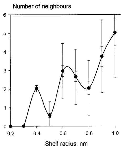
FIGURE 3 Histogram of an average number of C_\alpha atoms in 0.1 nm thick spherical shells around a given C_\alpha atom. Smaller error bars: variation of the averaged values over all proteins; larger error bars: averaged variation within one protein.
