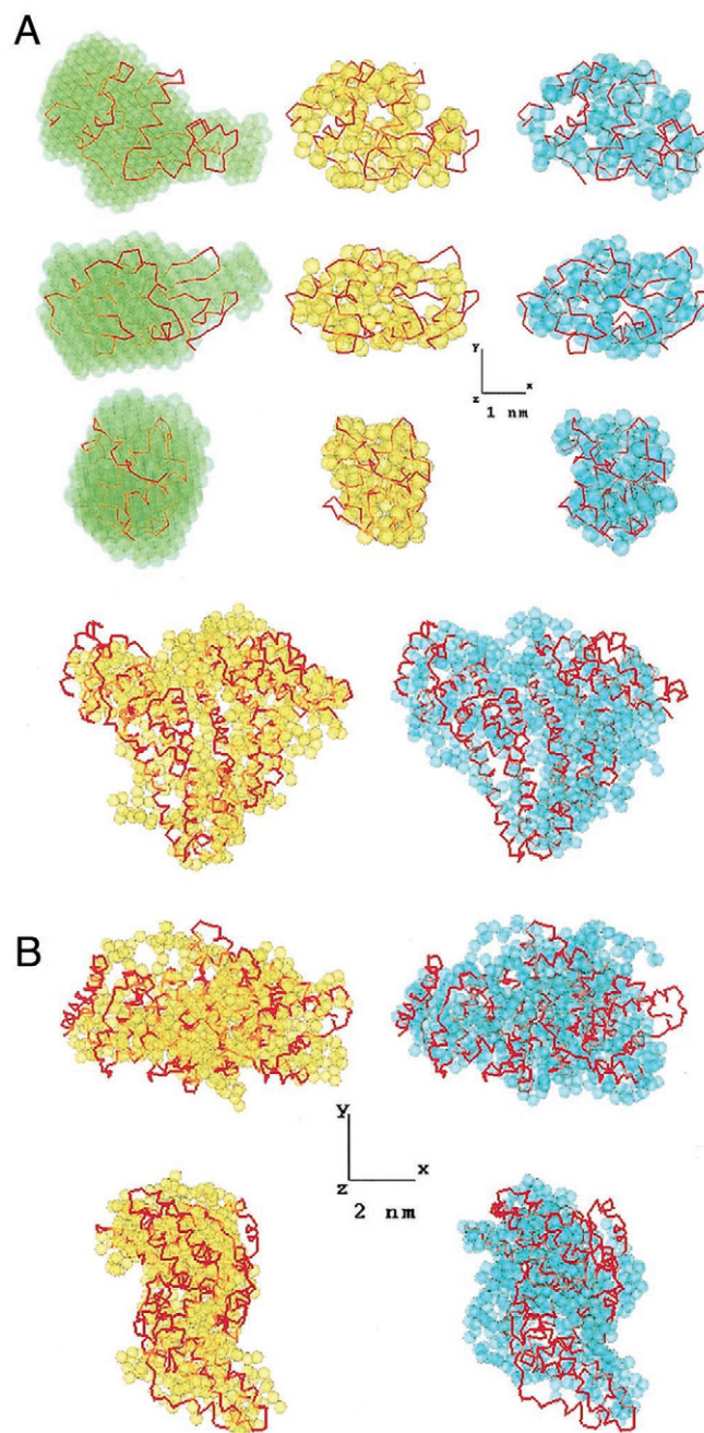
FIGURE 5 Atomic models of lysozyme ( A ) and ligand-bound HSA ( B ) superimposed with DR models from solution scattering. The atomic models are displayed as C_{\alpha} chains, DR models as semi-transparent spheres (yellow and cyan models yield best and worst agreement with the atomic model, respectively). For lysozyme, a low resolution shape obtained by DAMMIN (Svergun, 1999) is displayed in green (left column). The center and bottom rows are rotated counterclockwise by 90^{\circ} around X and Y, respectively. All three-dimensional models were displayed using the program ASSA (Kozin et al., 1997).
